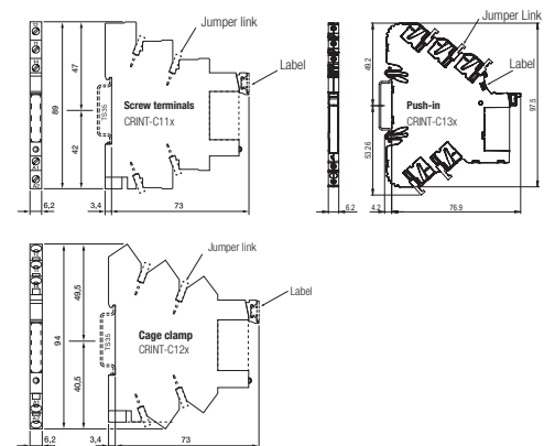
fig. 4. Dimension (mm)
