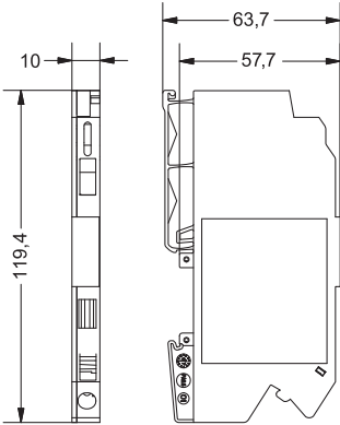
Dimensions Supply terminal
