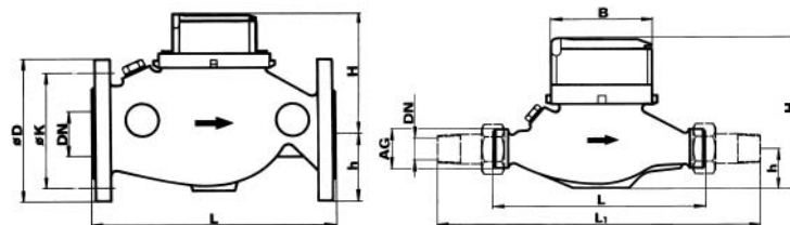
FLANGE DN 15-50/PN 16 AND DN 20-40/PN 40
